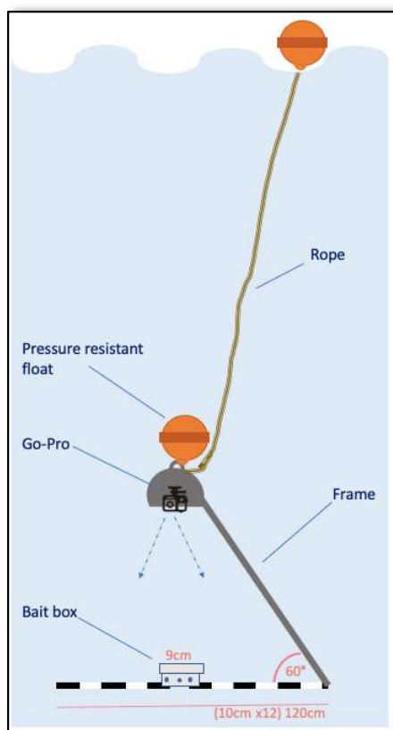
Figure 2 A diagram of the BUV apparatus
